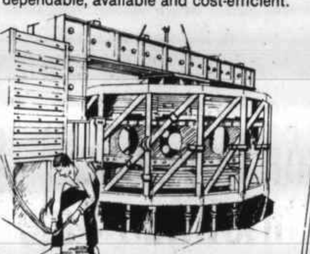
This is TEXT—the Texas Experimental Tokamak at the University of Texas Fusion Research Center in Austin. The machine will be used by scientists from throughout the nation to expand our knowledge of nuclear fusion.
